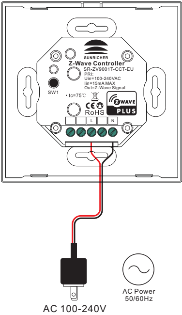
Wiring diagram
